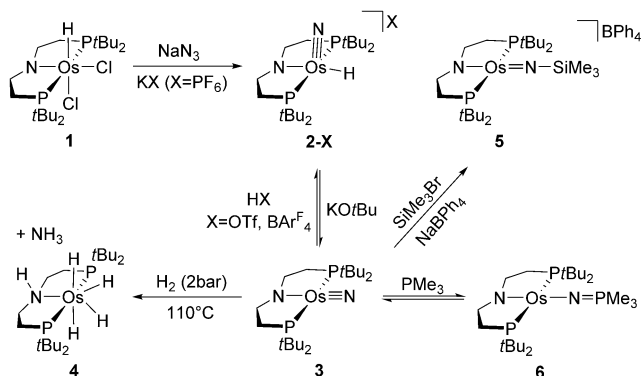
Scheme 2. Synthesis and reactivity of osmium(IV) nitride 3 ( \text{BARF}_4 = \text{B}(\text{C}_6\text{H}_3-3,5-(\text{CF}_3)_2)_4^- ).
